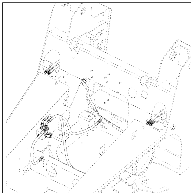
LOCATION REFERENCE - FLOAT CIRCUIT
